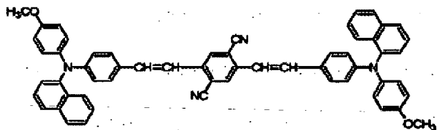
Structural formula (15)-12:
